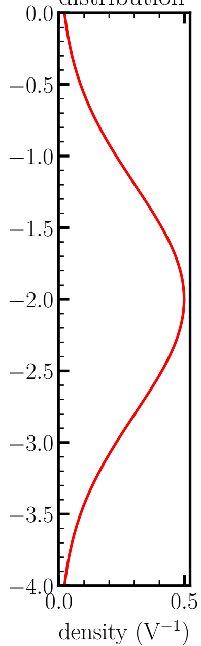
Marginal V_C^- distribution
