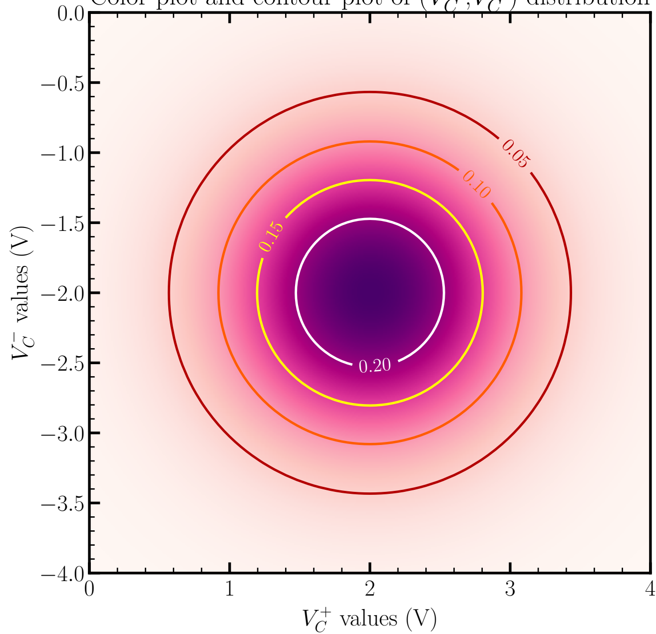
Color plot and contour plot of (V_C^+, V_C^-) distribution
